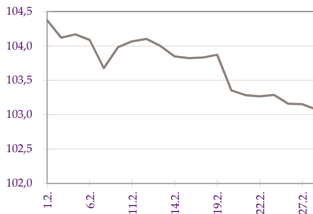
Chart 2: Zagreb Stock Exchange bond index CROBIS®
